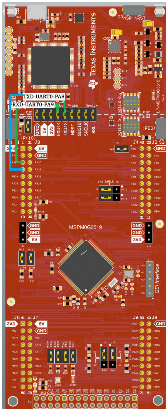
Figure 2-6. LP-MSPM0G3519 Backchannel Connection to UART0
