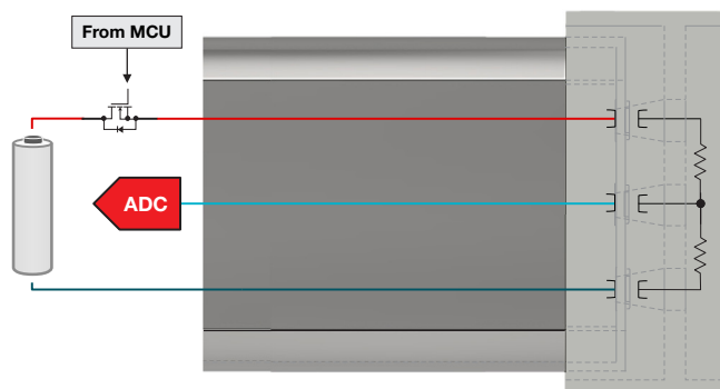
Figure 11. Deadbolt position sensing.
