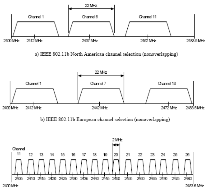
Figure 1: 2.4-GHz channels ( source: IEEE 802.15.4 standard )
