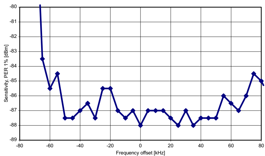
Figure 12. 500 kbps, MDMCFG2.DEM_DCFILT_OFF = 0
