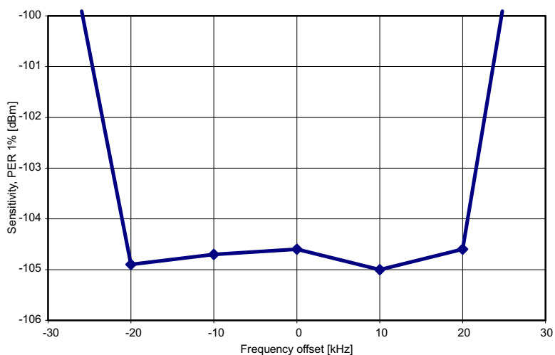
Figure 5. 4.8 kbps, MDMCFG2.DEM_DCFILT_OFF = 1
