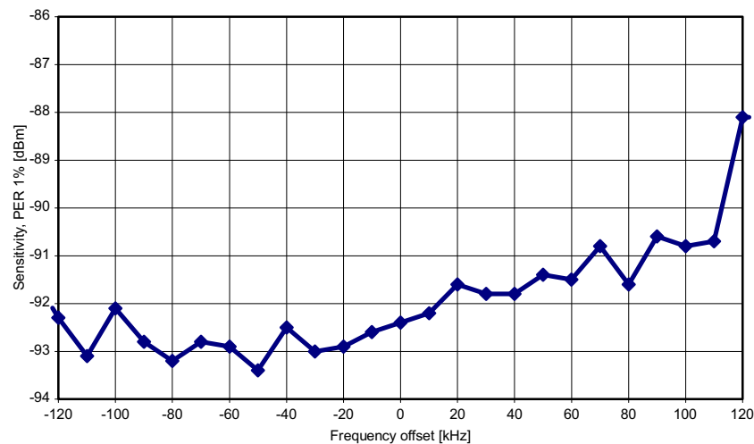
Figure 11. 250 kbps, MDMCFG2.DEM_DCFILT_OFF = 1
