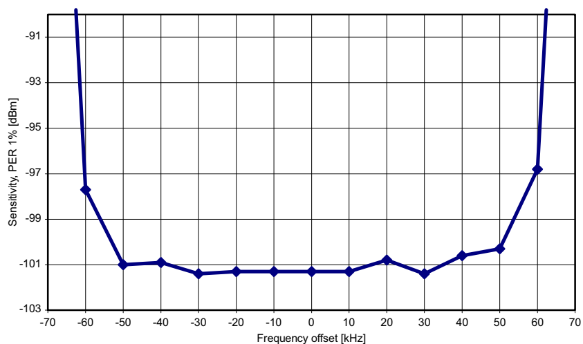
Figure 8. 38.4 kbps, MDMCFG2.DEM_DCFILT_OFF = 0
