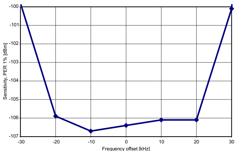
Figure 4. 4.8 kbps, MDMCFG2.DEM_DCFILT_OFF = 0
