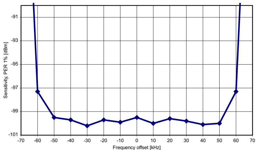
Figure 9. 38.4 kbps, MDMCFG2.DEM_DCFILT_OFF = 1
