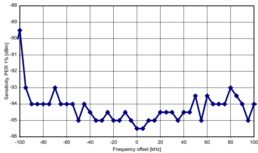
Figure 10. 250 kbps, MDMCFG2.DEM_DCFILT_OFF = 0
