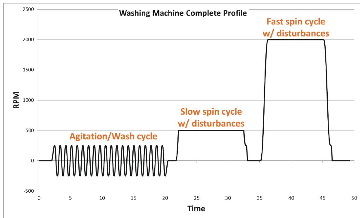
Figure 4-1. Washing Machine Profile
