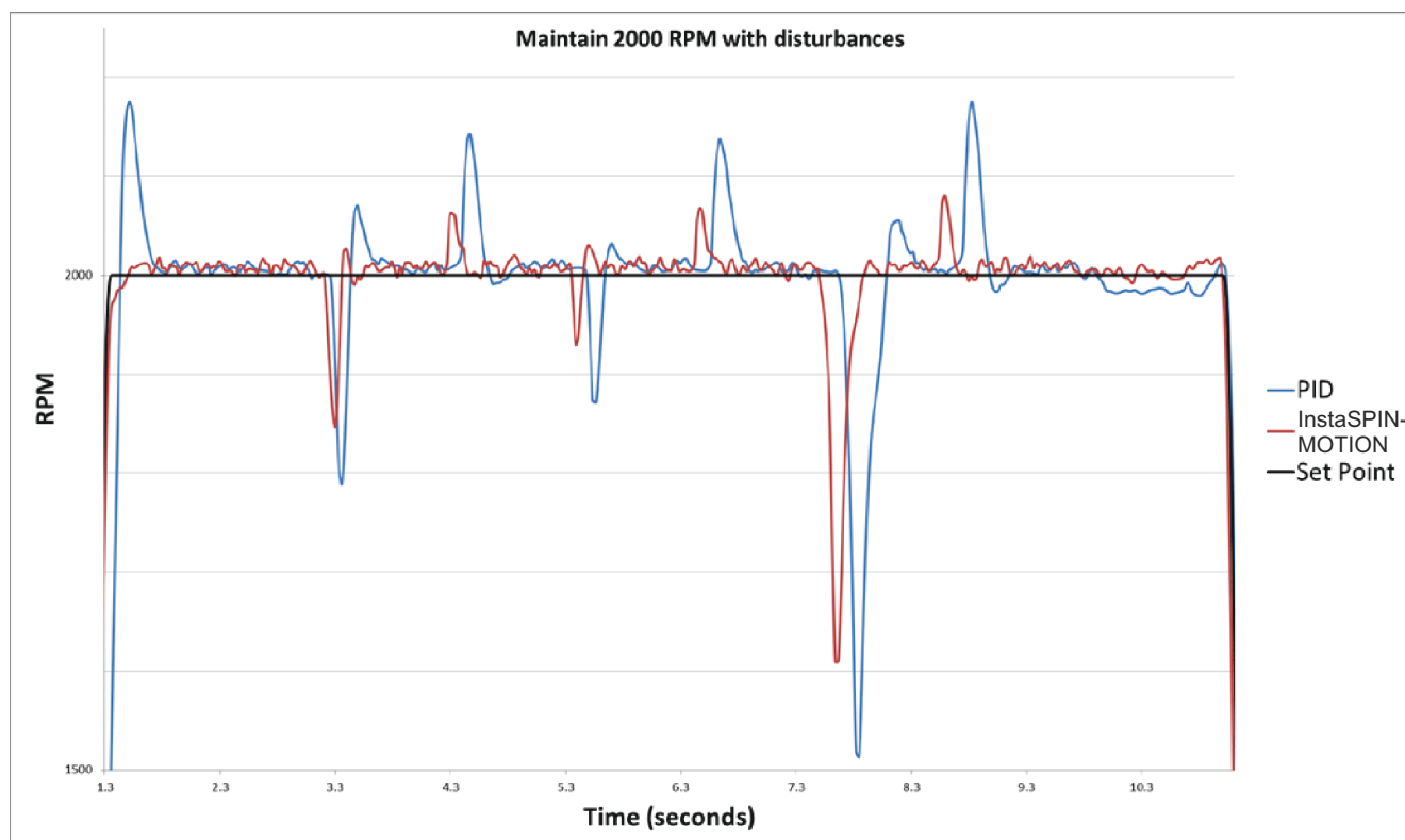
Figure 4-4. Second Spin Cycle - 2000 rpm
