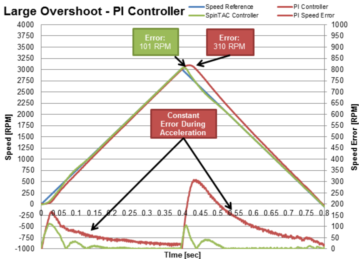
Figure 5-6. Large Overshoot for PI Controller During Reference Tracking
