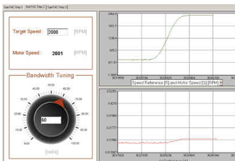
Figure 2-2. Simple Tuning Interface
