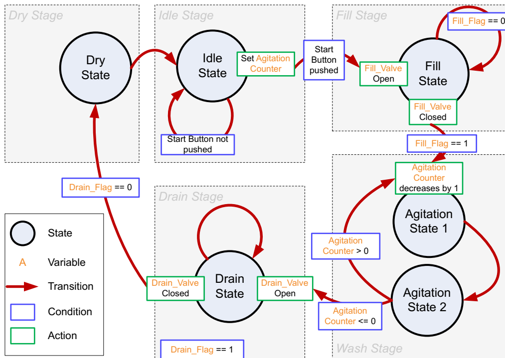
Figure 2-4. State Transition Map for a Washing Machine
