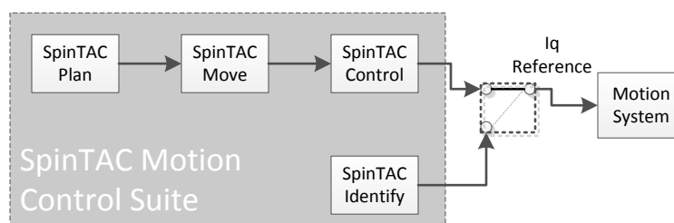
Figure 2-1. SpinTAC Motion Control Suite Components
