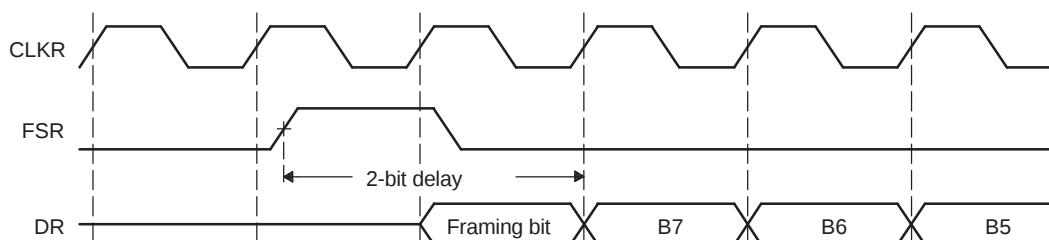
Figure 8-7. 2-Bit Data Delay Used to Skip a Framing Bit
