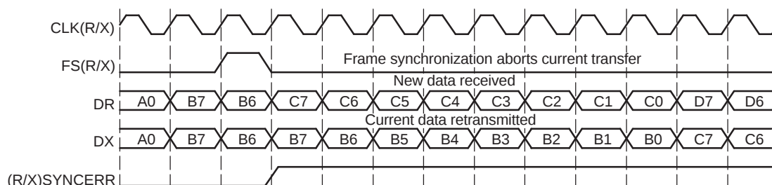
Figure 8-1. Unexpected Frame-Synchronization Pulse With (R/X) FIG = 0
