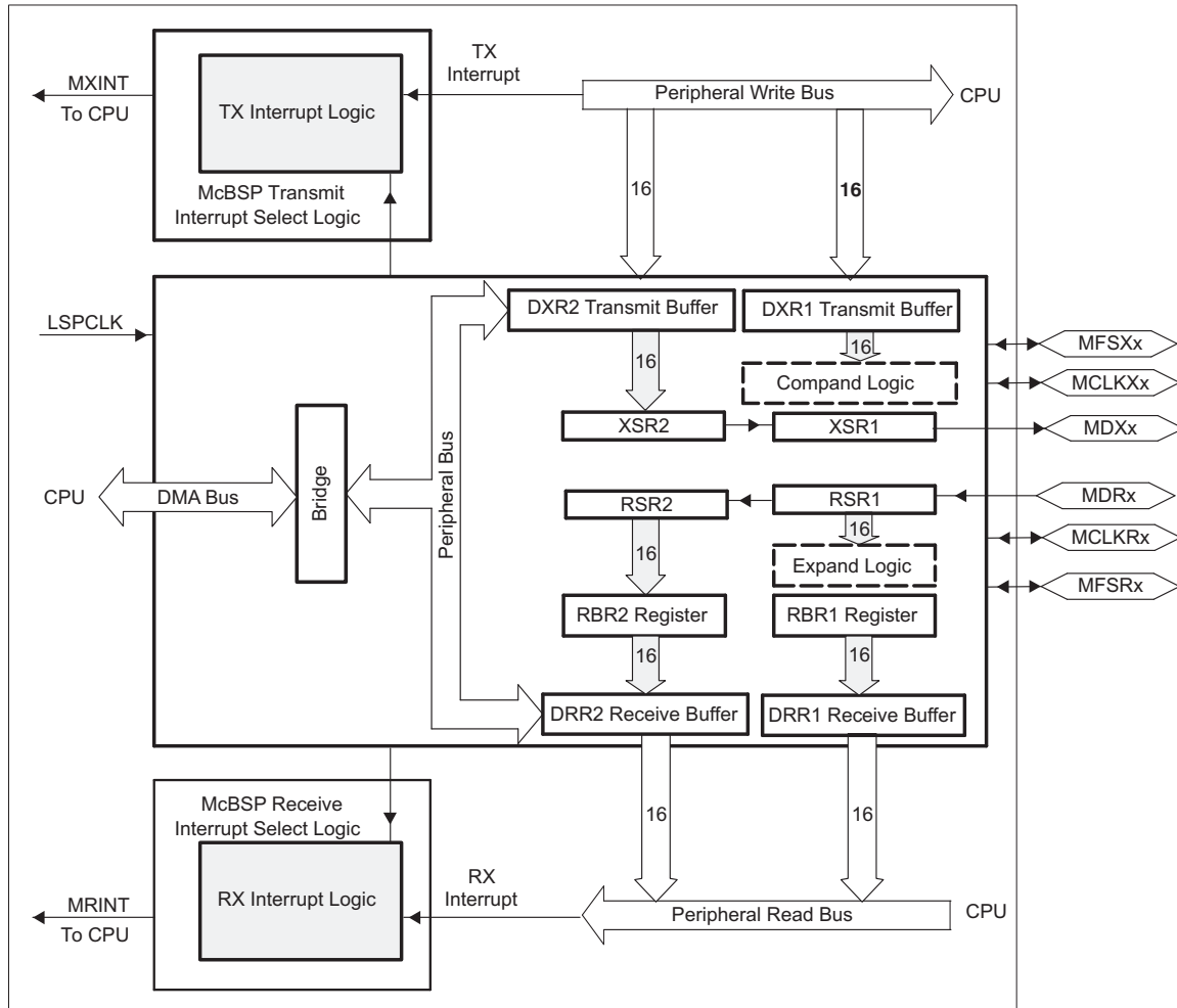
Figure 1-1. Conceptual Block Diagram of the McBSP
