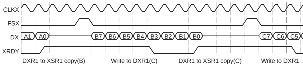
Figure 2-15. McBSP Transmission Signal Activity
