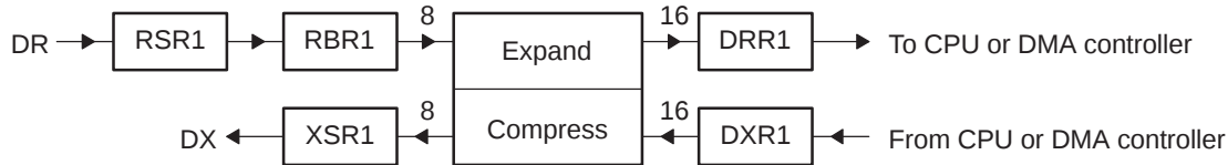
Figure 2-2. Companding Processes
