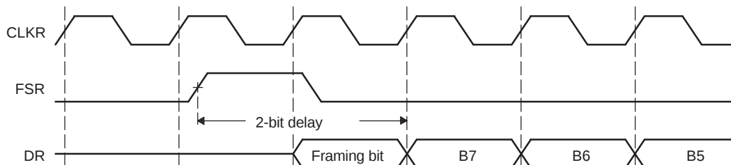
Figure 7-5. 2-Bit Data Delay Used to Skip a Framing Bit
