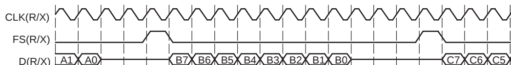
Figure 2-8. Single-Phase Frame for a McBSP Data Transfer
