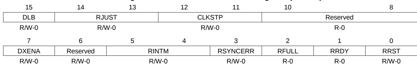
Figure 11-3. Serial Port Control 1 Register (SPCR1)
