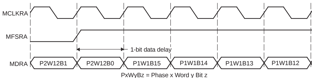
Figure 2-11. Timing of an AC97-Standard Data Transfer Near Frame Synchronization
