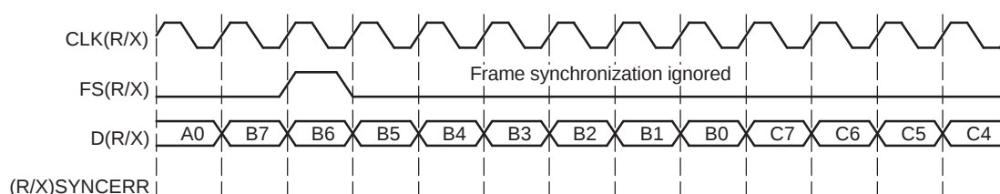
Figure 8-2. Unexpected Frame-Synchronization Pulse With (R/X) FIG = 1
