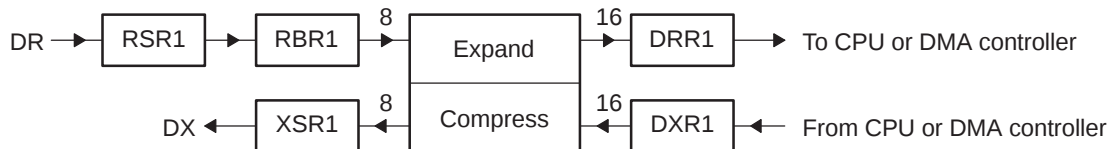
Figure 7-3. Companding Processes for Reception and for Transmission
