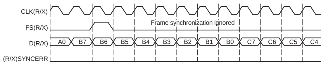
Figure 7-2. Unexpected Frame-Synchronization Pulse With (R/X)FIG = 1
