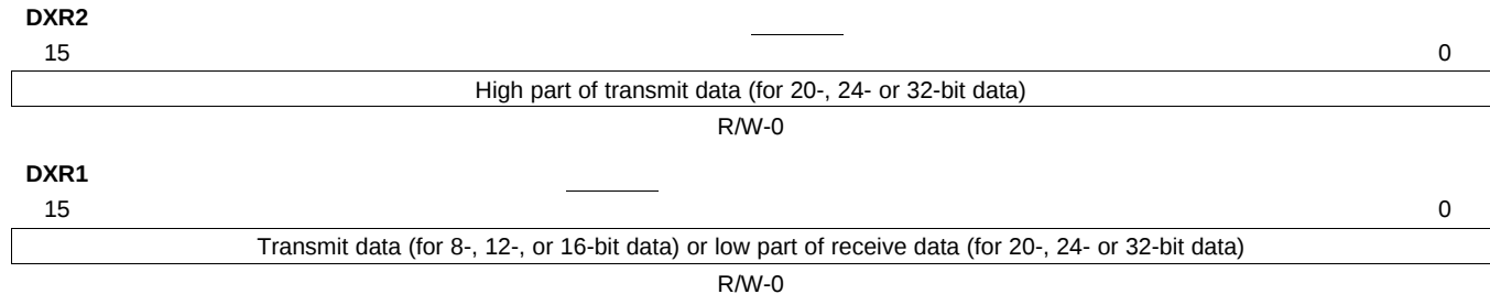
Figure 11-2. Data Transmit Registers (DXR2 and DXR1)
