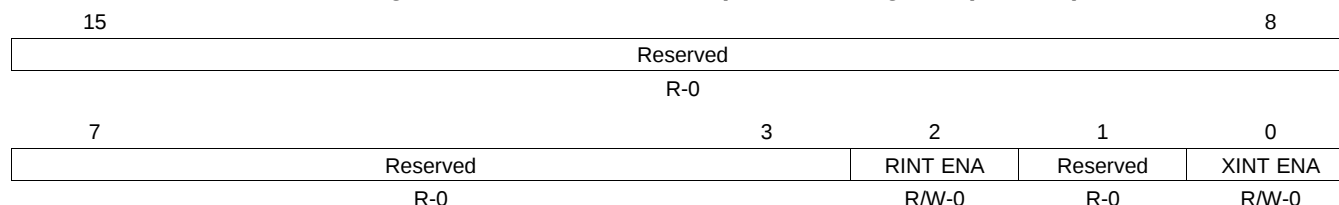
Figure 11-18. McBSP Interrupt Enable Register (MFFINT)
