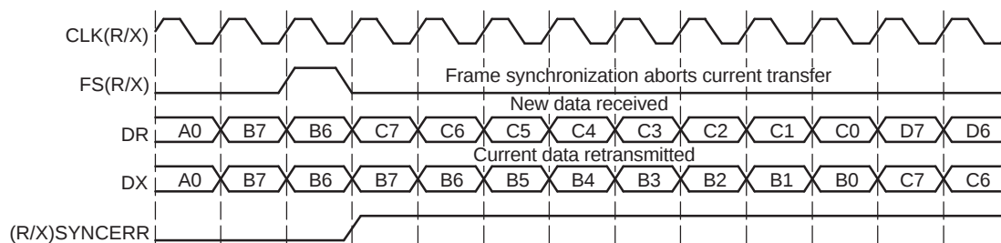
Figure 7-1. Unexpected Frame-Synchronization Pulse With (R/X)FIG = 0
