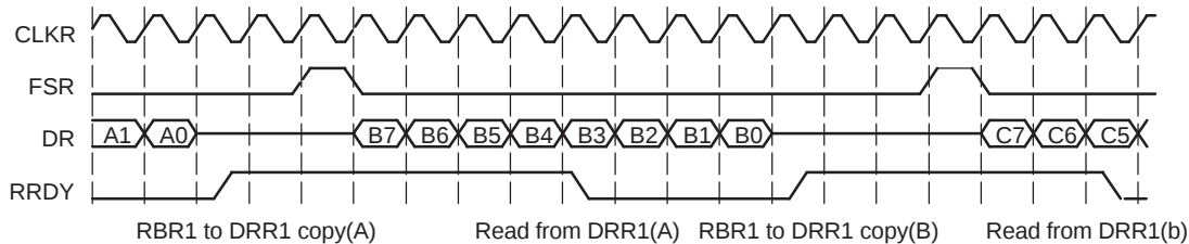
Figure 2-13. McBSP Reception Signal Activity
