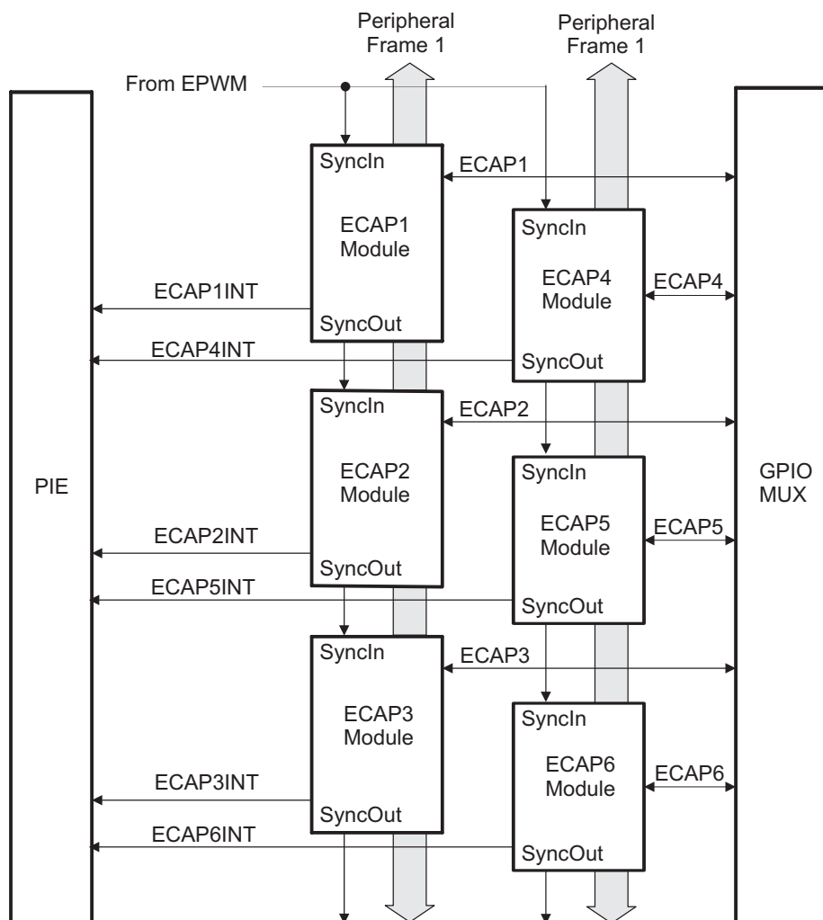
Figure 1. Multiple eCAP Modules In A 28034x System
