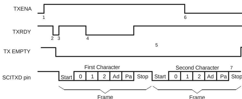
Figure 1-9. SCI TX Signals in Communications Mode
