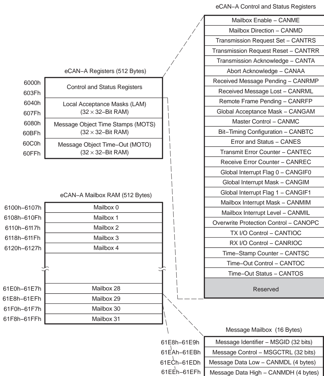
Figure 1-4. eCAN-A Memory Map
