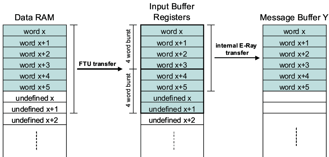
Figure 6. FTU Write Transfer of 6 Words
