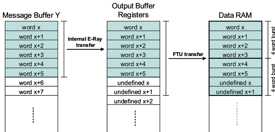
Figure 5. FTU Read Transfer of 6 Words
