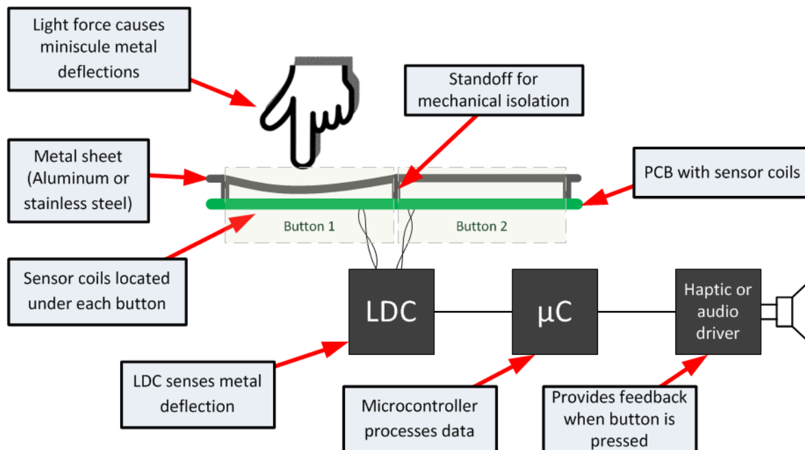
Figure 1. System Block Diagram of a Touch-On-Metal Implementation
