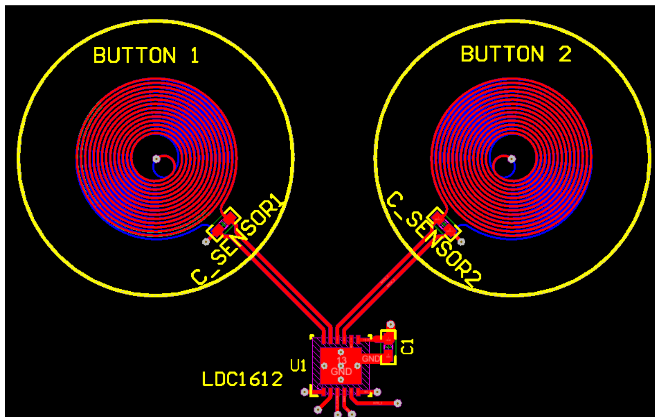
Figure 13. Sensor PCB (All Layers)
