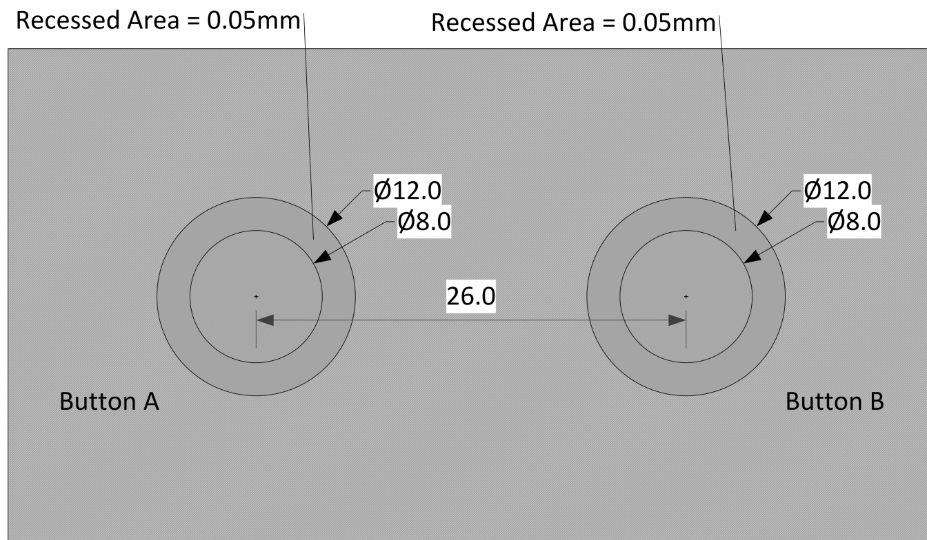
Figure 19. Top View
