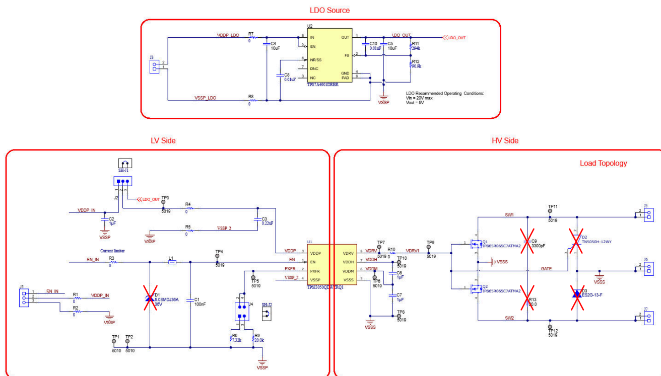
Figure 5-1. PSIL129 Schematic
