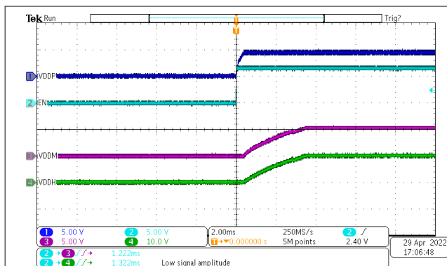
Figure 3-3. Two-Wire Mode Powering Up
