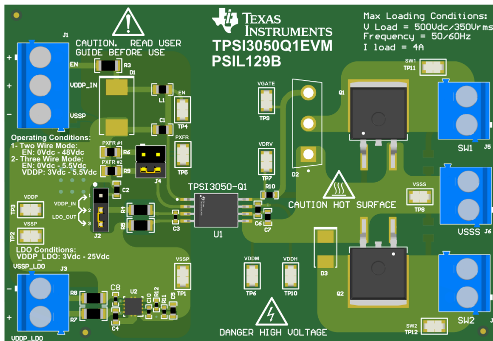
Figure 1-1. PCB View
