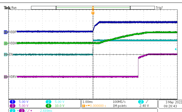
Figure 3-4. Two-Wire Mode Switching ON
