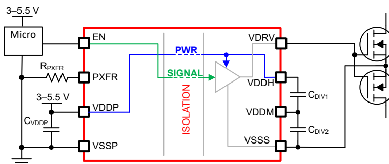
Figure 3-6. Three-Wire Mode Simplified Schematic
