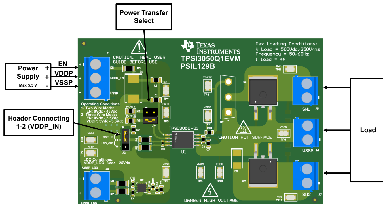
Figure 3-7. Three-Wire Mode VDDP Direct Supply
