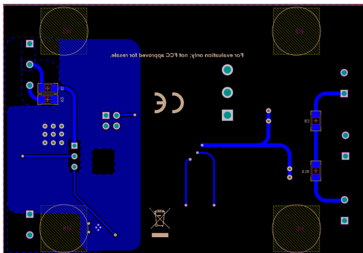
Figure 6-3. PCB Bottom Layer
