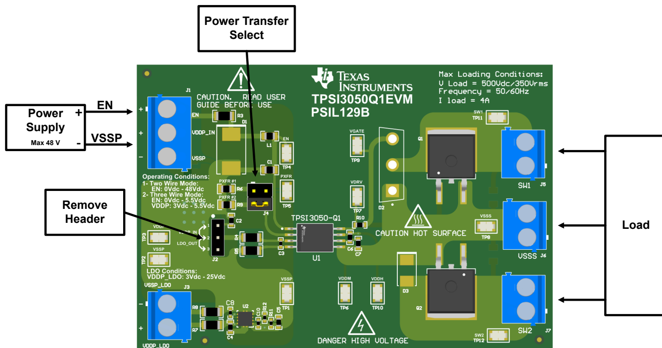
Figure 3-2. Two-Wire Mode Setup
