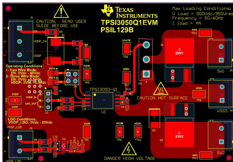
Figure 6-2. PCB Top Layer
