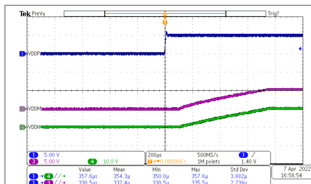
Figure 3-9. Three-Wire Mode Powering Up
