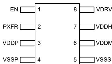
Figure 1-3. TPSI3050-Q1, TPSI3050S-Q1 DWZ Package 8-Pin SOIC Top View
