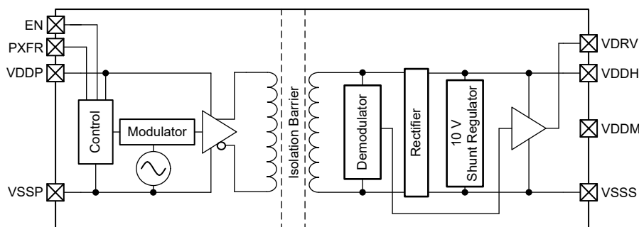
Figure 1-2. TPSI3050-Q1 Functional Block Diagram
