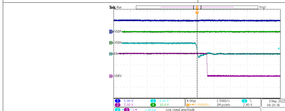
Figure 3-11. Three-Wire Mode Switching OFF
