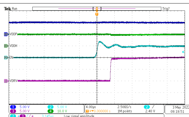
Figure 3-10. Three-Wire Mode Switching ON
