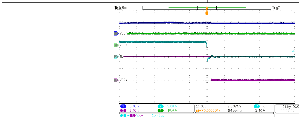
Figure 3-5. Two-Wire Mode Switching OFF
