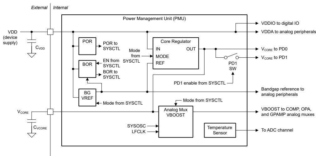
Figure 6-4. Power Module of MSPM0G
