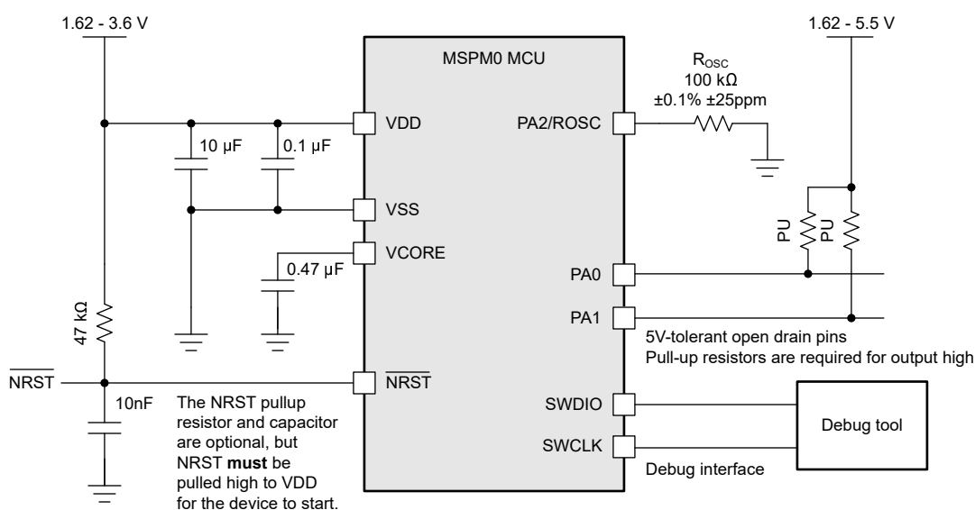
Figure 3-1. Basic Application Schematic of MSPM0G
