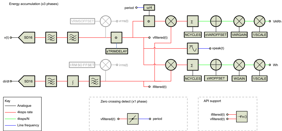
Figure 5. Software Flowchart
