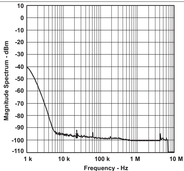
Figure 7. Output With RC Low-Pass Filter (1 kΩ and 4.7 nF) in Series Between the Output and Analyzer
