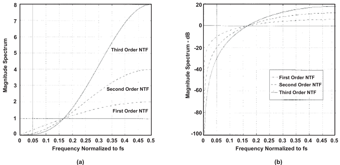
A 1^2 NTF for the first, second, and third order \Sigma\Delta modulators; (a) magnitude spectra on a linear scale. For comparison, the oversampled PCM NTF, which has a unity gain is shown; (b) magnitude spectra in dB.
