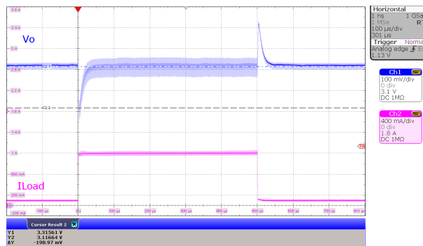
Figure 10-22. Load Transient, PFM/PWM Buck-Boost Operation
