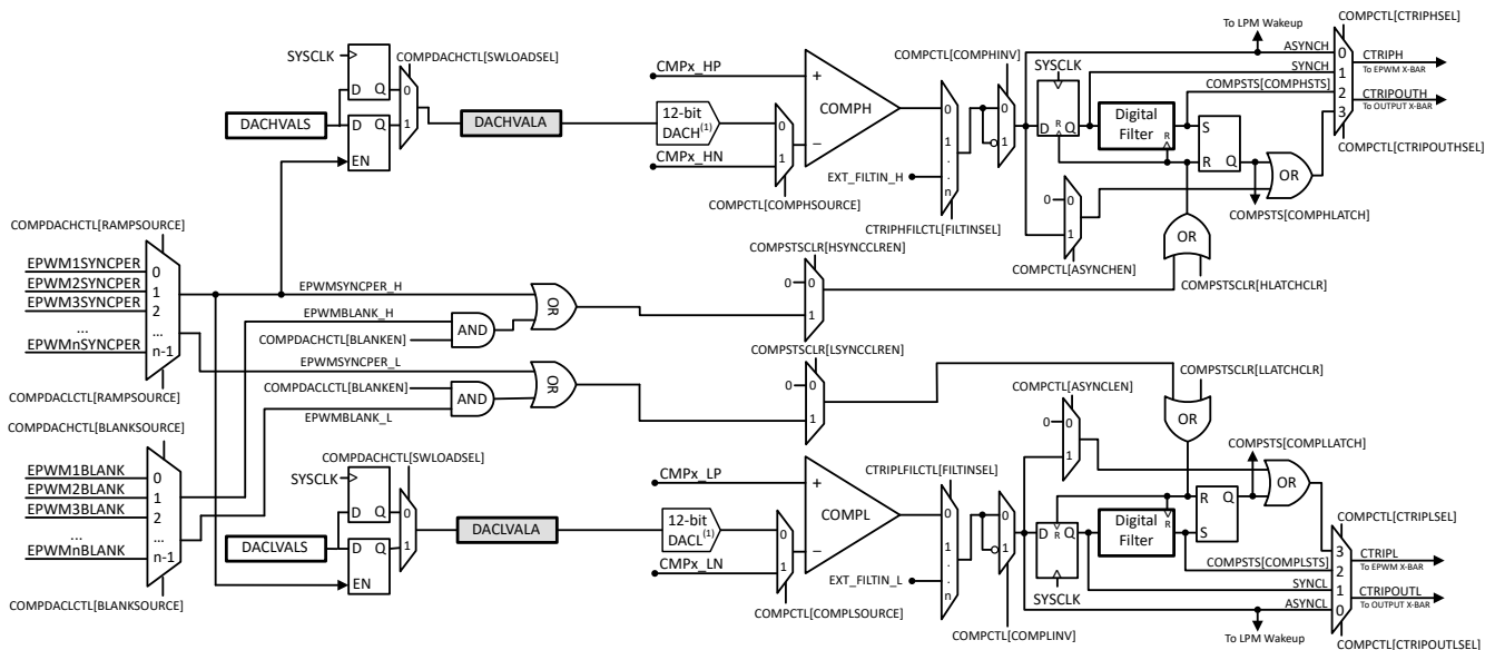
Figure 6-44. CMPSS Module Block Diagram
