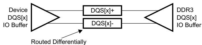
Figure 8-27. DQS[x] Topology
