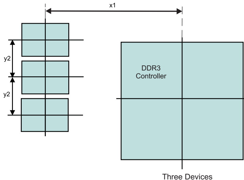
Figure 8-47. Placement Specifications
