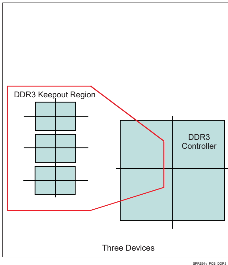
Figure 8-48. DDR3 Keepout Region
