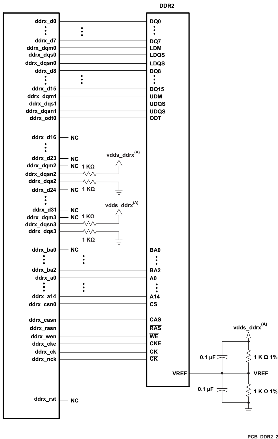
Figure 8-39. 16-Bit DDR2 High-Level Schematic
