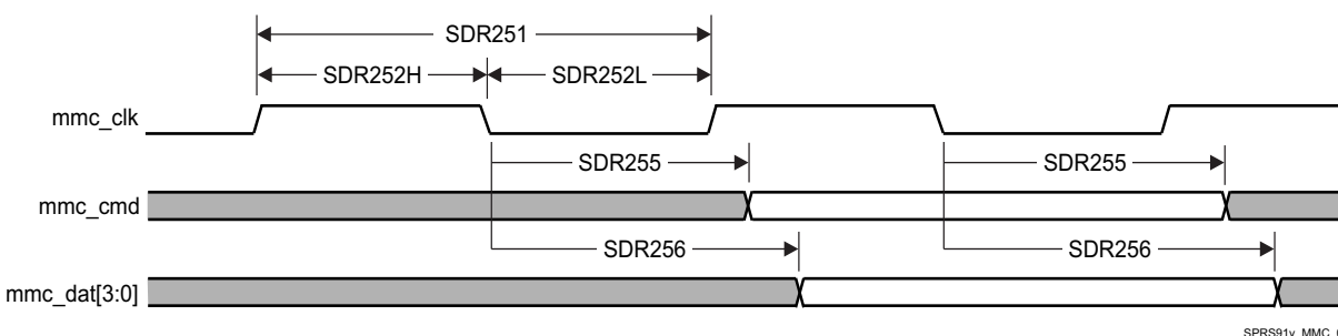
Figure 7-46. MMC/SD/SDIOj in - SDR25 - Transmitter Mode
