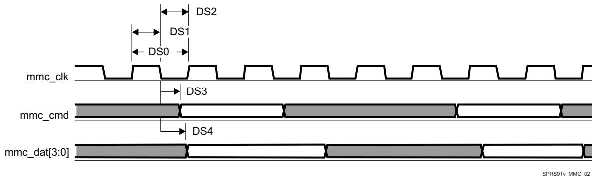
Figure 7-40. MMC/SD/SDIOj in - Default Speed - Transmitter Mode
