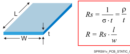
Figure 8-4. Static IR Drop Budget for PCB Only
