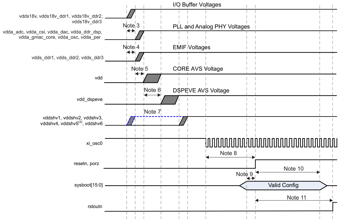
Figure 5-1. Power-Up Sequencing
