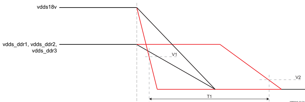
Figure 5-4. vdds18v and vdds_dds* Discharge Relationship (1)
