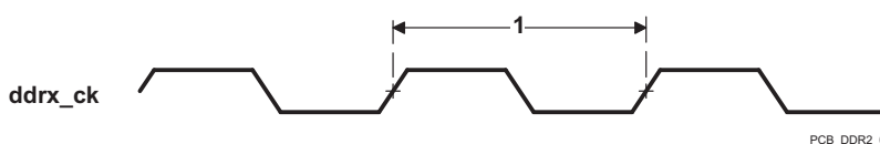
Figure 8-37. DDR2 Memory Controller Clock Timing
