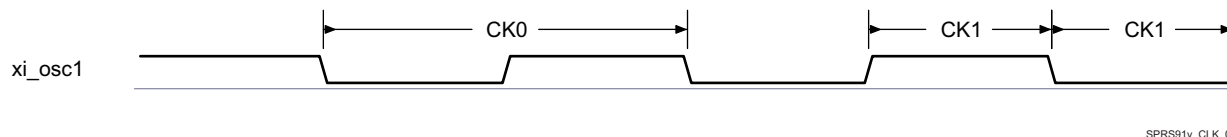
Figure 6-9. xi_osc1 Input Clock
