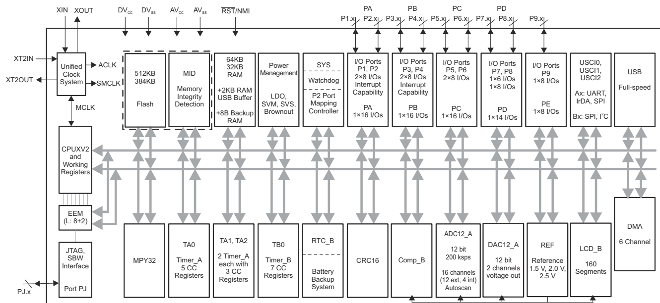
Functional Block Diagram – MSP430F6659, MSP430F6658
