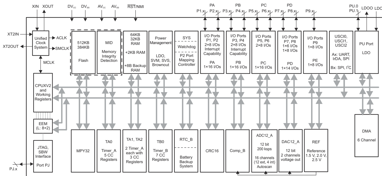
Figure 4-3. Functional Block Diagram – MSP430F5359, MSP430F5358
