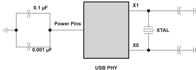
Figure 7-25. Power Supply and Clock Connection to the USB PHY
