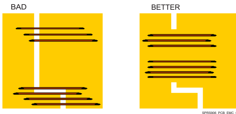
Figure 7-11. Trace Examples
