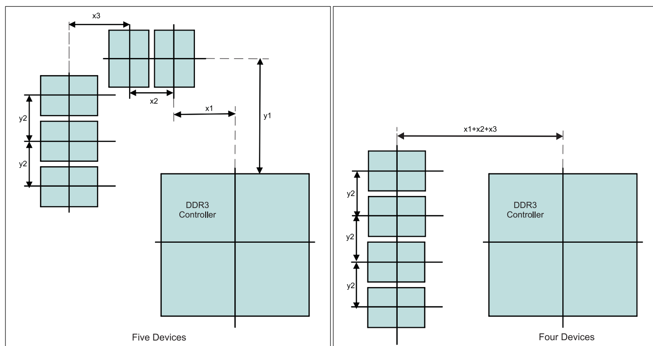
Figure 7-40. Placement Specifications
