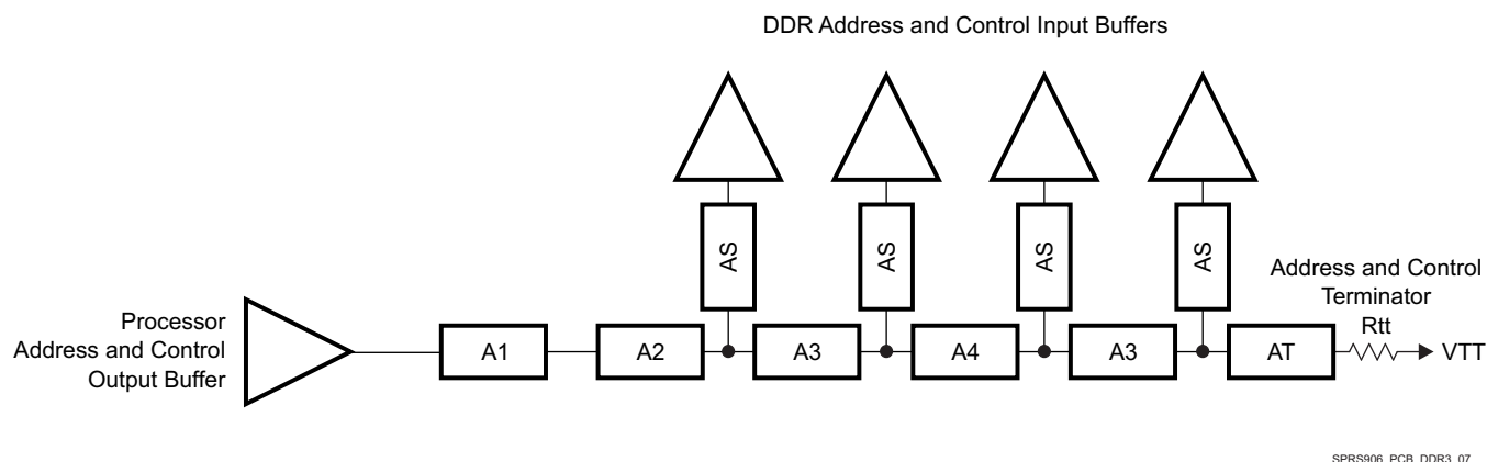
Figure 7-43. ADDR_CTRL Topology for Four x8 DDR3 Devices
