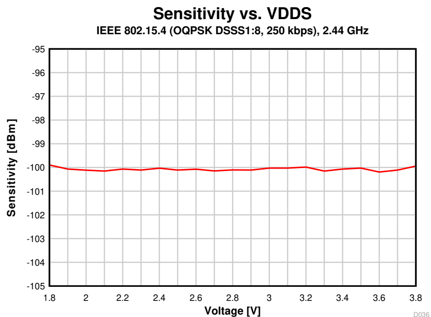
Figure 8-33. Sensitivity vs. Supply Voltage (VDDS) (250 kbps, 2.44 GHz)
