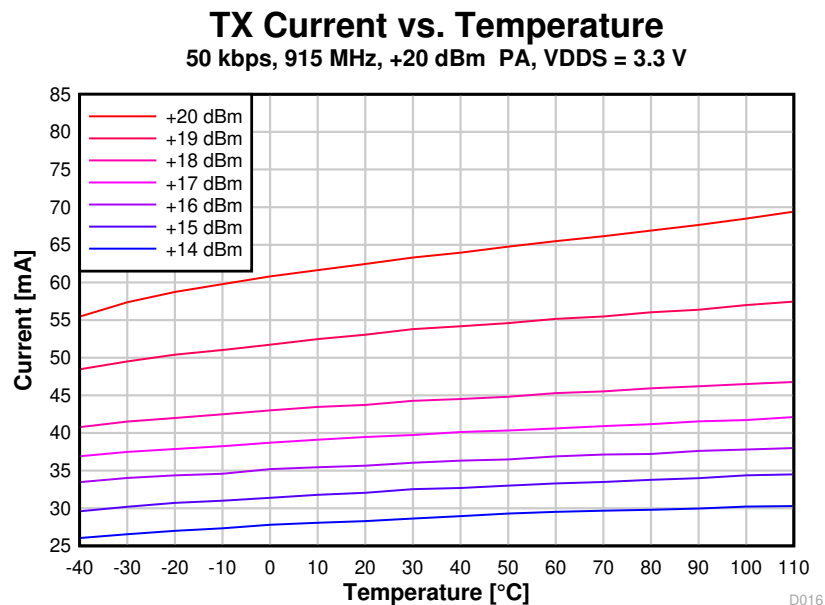
Figure 8-14. TX Current vs. Temperature (50 kbps, 915 MHz, VDDS = 3.3 V)
