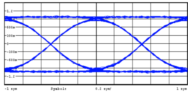
Figure 4-14. Eye Diagram
