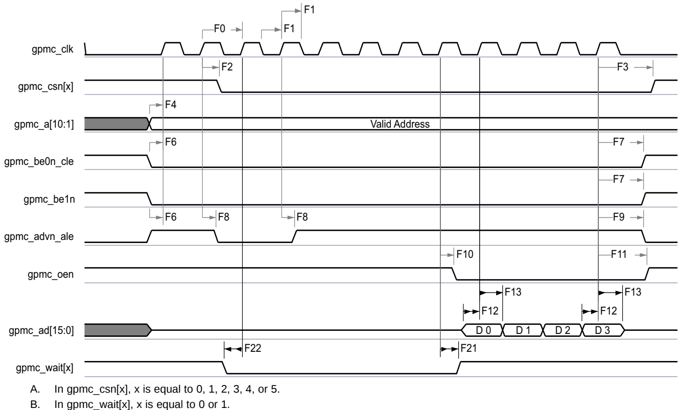
Figure 7-18. GPMC and NOR Flash—Synchronous Burst Read—4x16-Bit (GpmcCLKDivider = 0)
