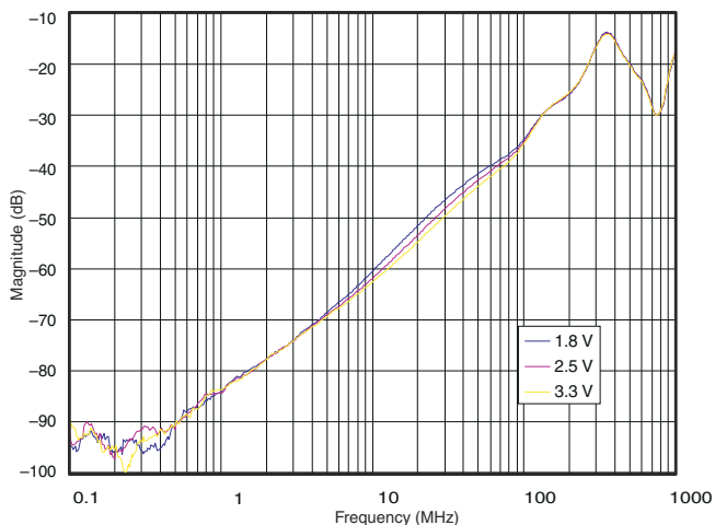
Figure 6-8. Crosstalk
