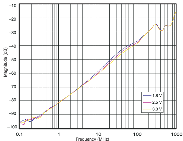
Figure 6-10. OFF Isolation
