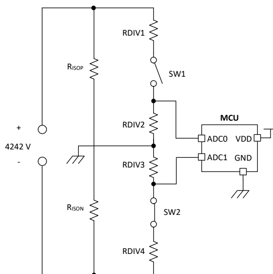
Figure 2. Insulation monitoring high-potential example
