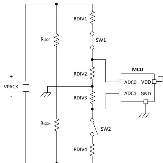
Figure 1. Insulation monitoring configuration
