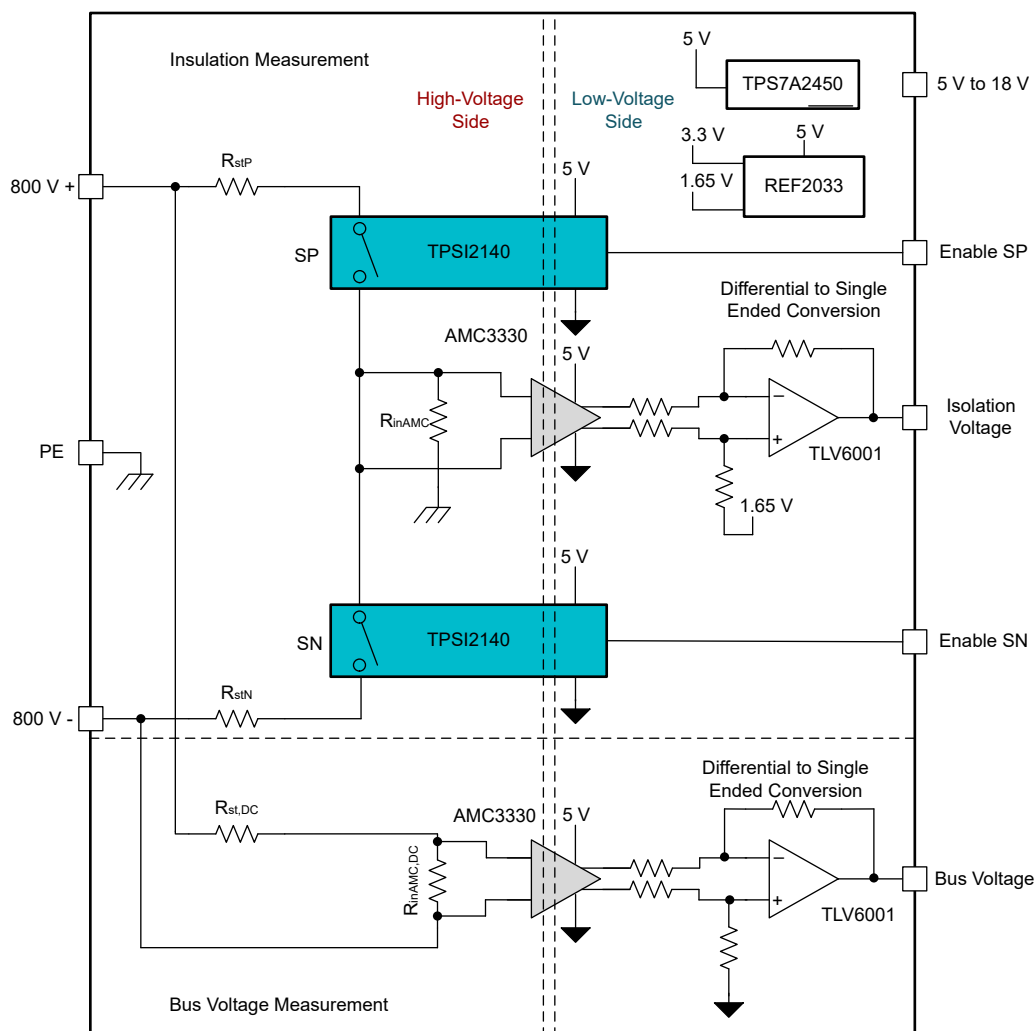
Figure 4. AFE reference design block diagram
