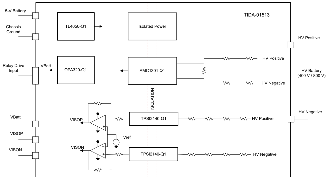
Figure 5. Leakage measurements reference design block diagram
