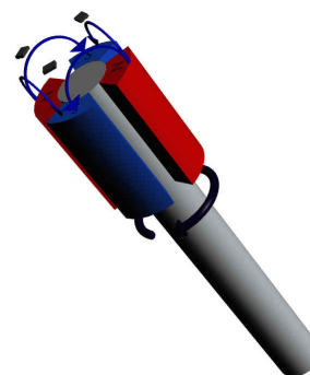
Figure 7. Rotor Position Using Surface Mount Hall Sensor
