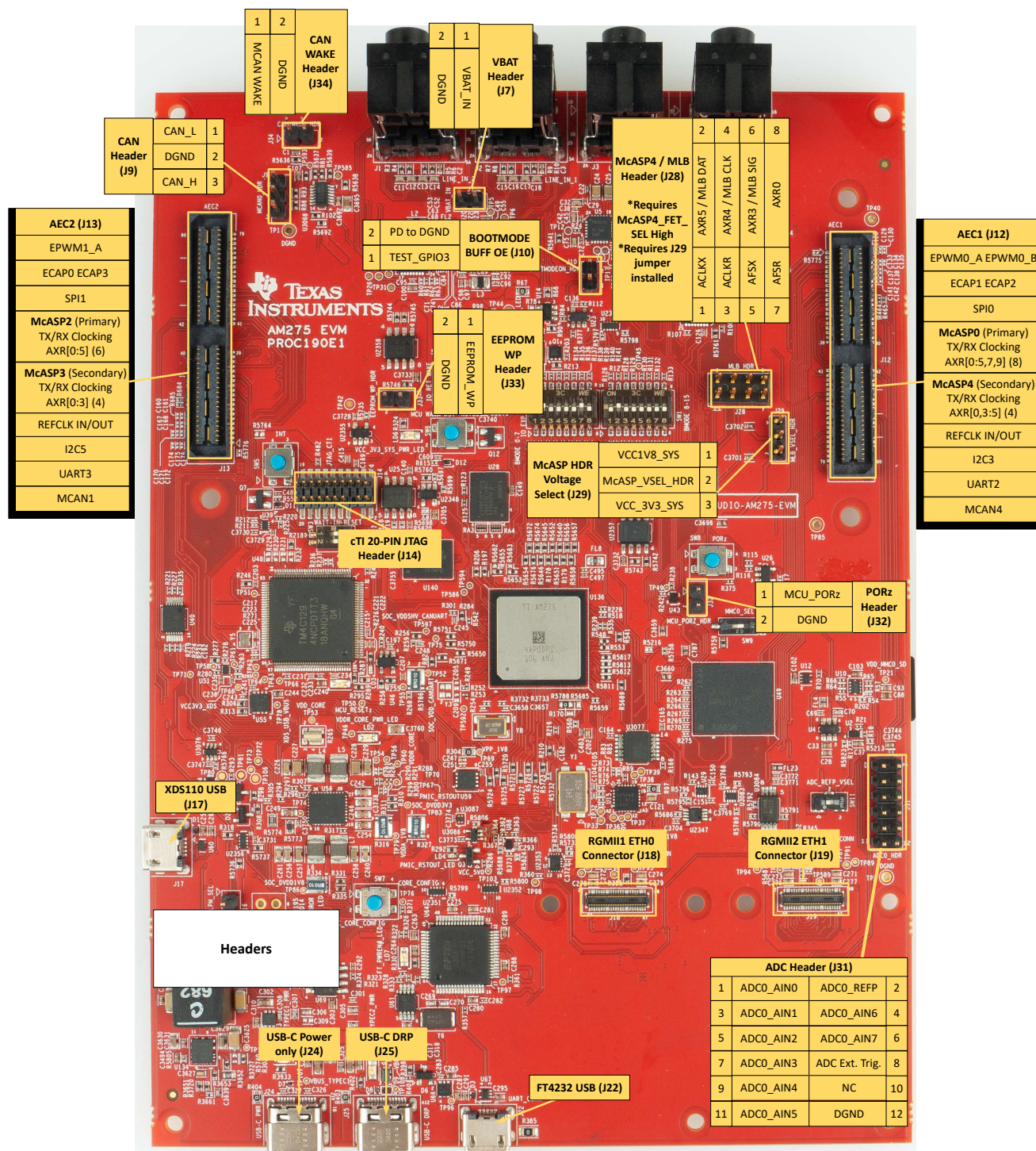
Figure 2-18. Headers
