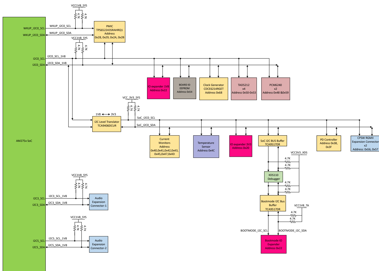
Figure 2-32. I2C Interface Tree
